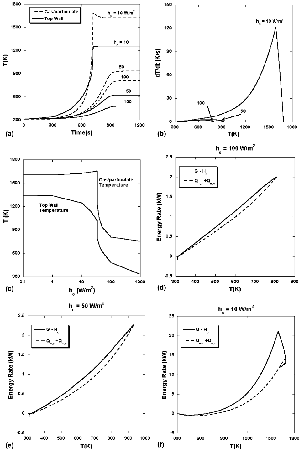
Fig. 3. (a) Temperature of the hot layer and top wall for W_v = 0.2 m and f_{v,0} = 10^{-7} with different external heat transfer coefficient. (b) Rate of the hot layer temperature increase for W_v = 0.2 m and f_{v,0} = 10^{-7} with different external heat transfer coefficient. (c) Steady state temperature for W_v = 0.2 m and f_{v,0} = 10^{-7} with different external heat transfer coefficient. Behavior of the dependence of energy rates on the hot layer temperature for W_v = 0.2 m, f_{v,0} = 10^{-7} : (d) h_o = 100 W/m^2 , (e) h_o = 50 W/m^2 and (f) h_o = 10 W/m^2 .
