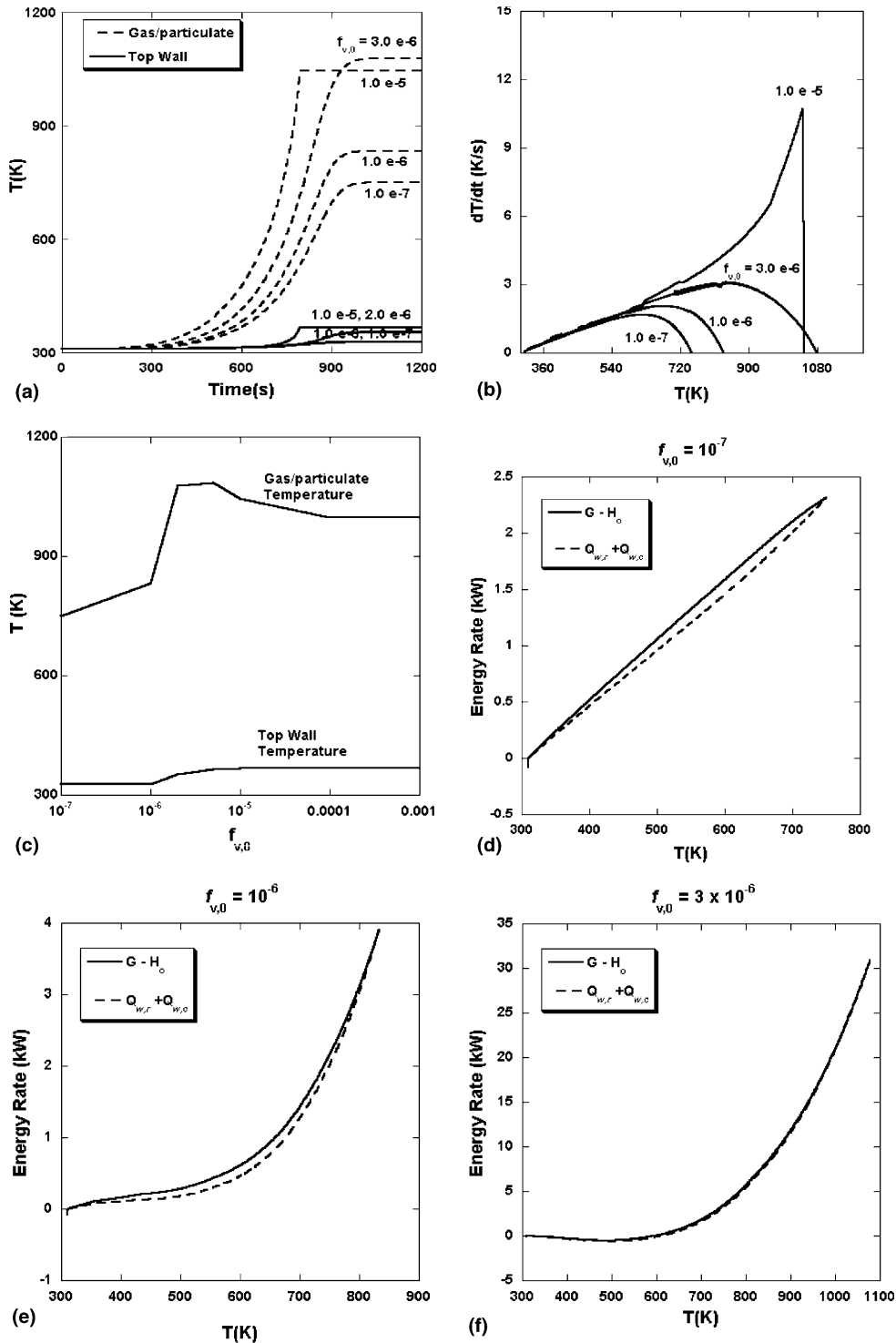
Fig. 4. (a) Temperature of the hot layer and top wall for W_v = 0.2 m and h_o = 1000 W/m 2 with different particulate volume fraction. (b) Rate of the hot layer temperature increase for W_v = 0.2 m and h_o = 1000 W/m 2 with different particulate volume fraction. (c) Steady state temperature for W_v = 0.2 m and h_o = 1000 W/m 2 with different particulate volume fraction. Behavior of energy rates for W_v = 0.2 m, h_o = 1000 W/m 2 : (d) f_{v,0} = 10^{-7} , (e) f_{v,0} = 10^{-6} and (f) f_{v,0} = 3 \times 10^{-6} .
