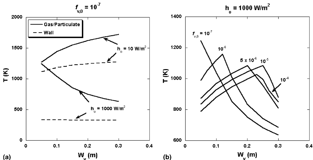
Fig. 5. (a) Temperature of the hot layer and the wall at different external heat transfer coefficient and vent width. (b) Temperature of the hot layer at different particulate volume fraction and vent width (the wall temperature is at 300 K due to the high external heat transfer coefficient).
