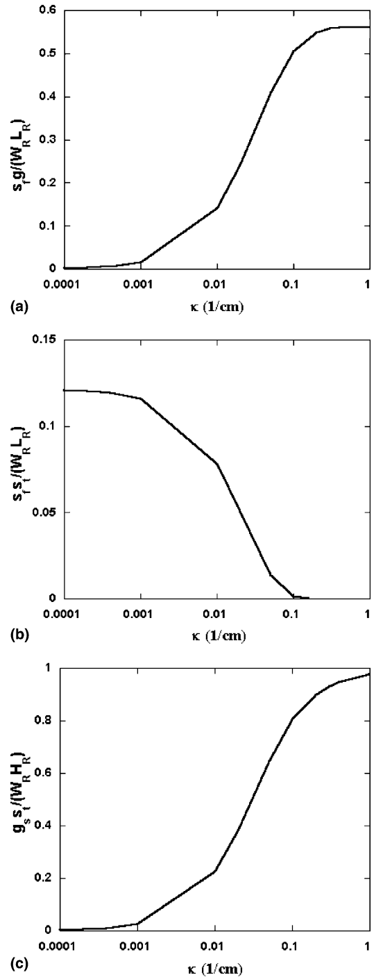
Fig. 2. Exchange factor (a) between the fire base and the hot layer, (b) between the fire base and the top wall and (c) between the hot gas layer and the top wall (with W_R = L_R = H_R = 40 cm, L_f = 30 cm, and Z_d = 0 ).
