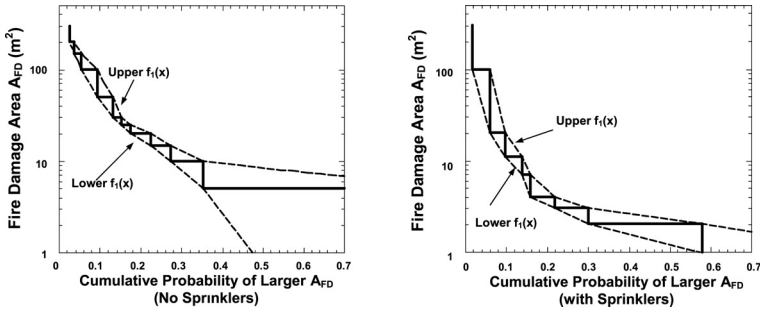
Figure 6 The upper bound and lower bound of the cumulative probability distribution, f_1(x) for the sprinklered and unsprinklered cases
