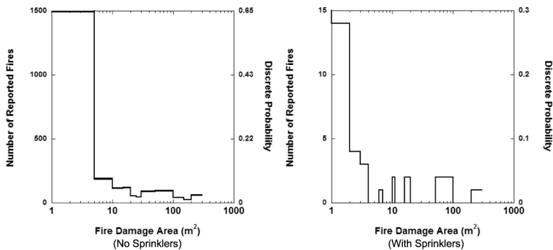
Figure 1 Number distributions and the corresponding discrete probability Distributions of reported fires for office premises with and without sprinklers
