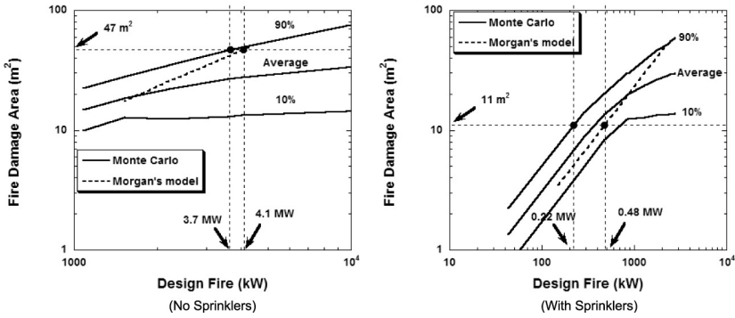
Figure 12 The variation of fire damage area with design fires accounting for the variation of parameters as represented by equations (7), (11), (13) and (14)
