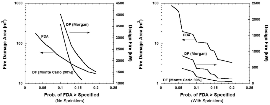
Figure 13 Fire damage area and design fire using the Morgan’s approach and the Monte Carlo approach
