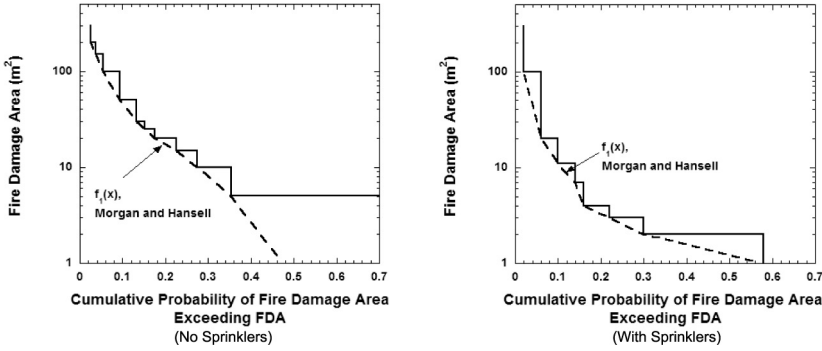
Figure 2 Cumulative probability distributions for reported fires for office premises with and without sprinklers (The broken line represents the cumulative probability function, f_1(x) , as utilized by Morgan and Hansell [12])
