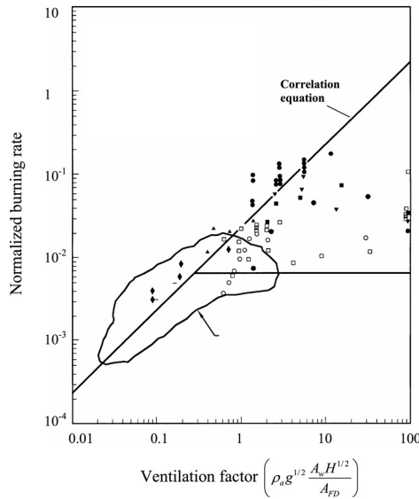
Figure 8 Data for transition from a ventilation-controlled fire to a fuel-bed controlled fire for various fuels (e.g. [20])
