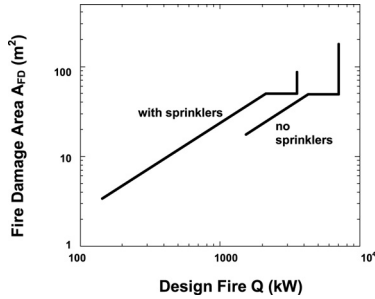
Figure 4 Relation between fire damage area and design fire according to equations (4), (5a) and (5b) with H = 3\text{ m} , A_w = 9\text{ m}^2
